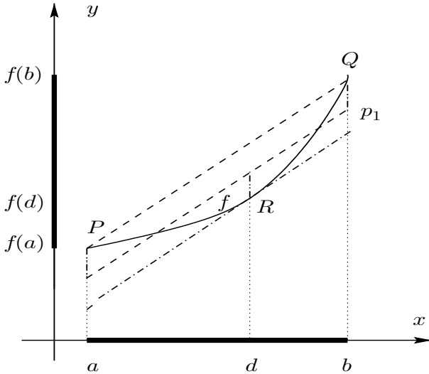
Fig. 8.3. Construction of minimax polynomial of degree 1.
