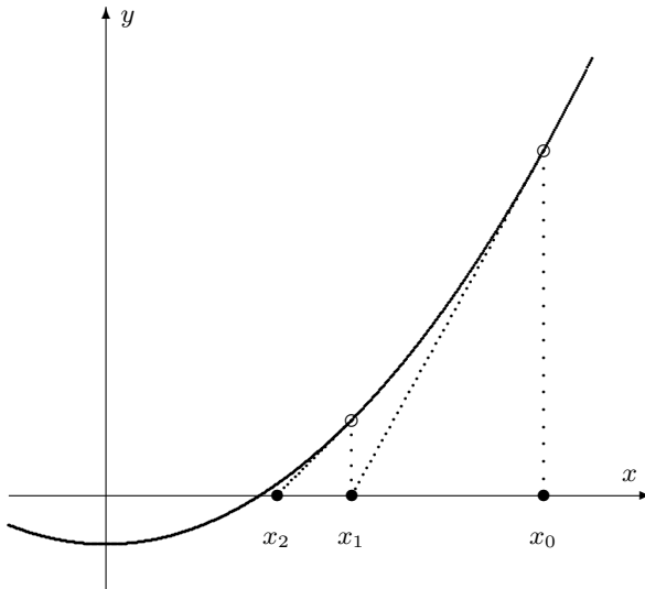
Fig. 1.5. Newton's method.
